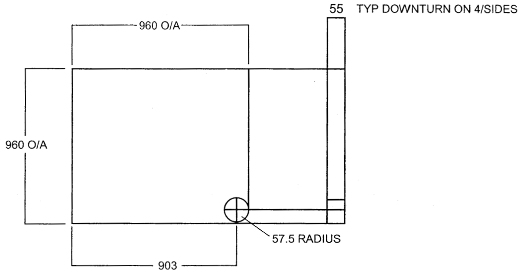
LANDING DETAIL
