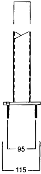
HANDRAIL POST BASE
